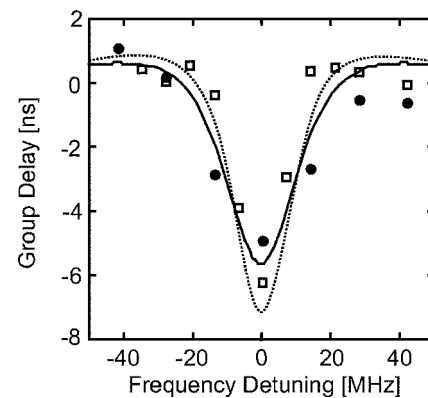
FIG. 4. The solid circles and open squares are observed delay time as a function of the frequency detuning, in the resonance line of 70 MHz (shown in Fig. 2) and 60 MHz, respectively. The solid and dotted curves are the theoretical calculated delay time.
